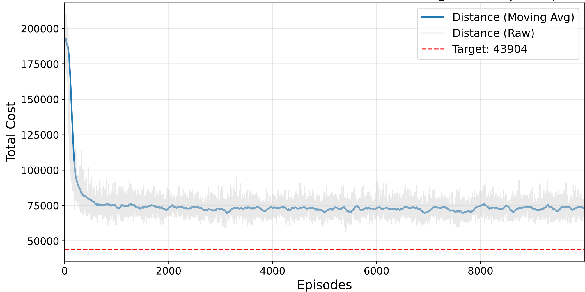
Final HYPERBAND TPE Masked AutoRL-SOP Training - kro124p.3.sop
